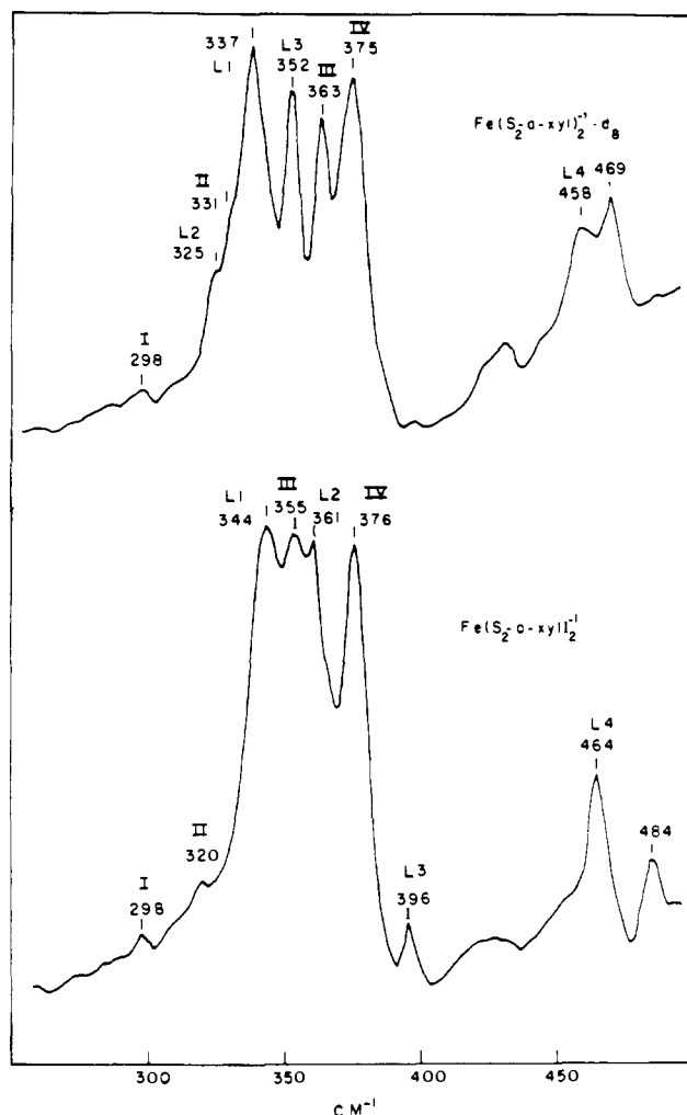
Figure 3. Infrared spectra of Fe(S 2 -o-xylyl) 2 - and Fe(S 2 -o-xylyl) 2 - -d 8 , obtained with Nujol nulls between polyethylene plates, by using a Digilab FTIR spectrometer, at 4-cm -1 resolution. Bands assigned to Fe-S stretching and to ligand modes are labeled I-IV and L1-L4.
