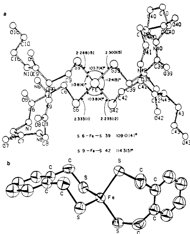
Figure 7. (a) A stereo view of the active site of oxidized rubredoxin from C. pasteurianum , adapted from ref 25. It illustrates the presence of a C_2 axis and the two pairs of Fe-S-C-C dihedral angles, \sim 90^\circ and \sim 180^\circ . (b) ORTEP drawing of the molecular structure of \text{Fe}(\text{S}_2\text{-}o\text{-xylyl})_2^- (from ref 28), viewed down the C_2 axis. The dihedral angles about the -S-C bonds are all close to 90^\circ .
