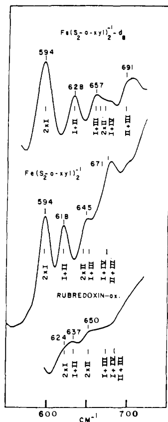
Figure 2. Fe-S overtone region Raman spectra of D. gigas Rd ox (2.0 mM in 0.1 M Tris-HCl buffer, pH 7.4) and of (Et 4 N)[Fe(S 2 -o-xylyl) 2 ] (~4 mM in acetonitrile). All spectra were obtained via backscattering from sealed spinning NMR tubes cooled with cold N 2 gas by using a 4880-Å Ar + excitation (150 mW) and 10 cm -1 slit width. Expected positions of the I-IV overtones and combination levels are marked with horizontal lines.
